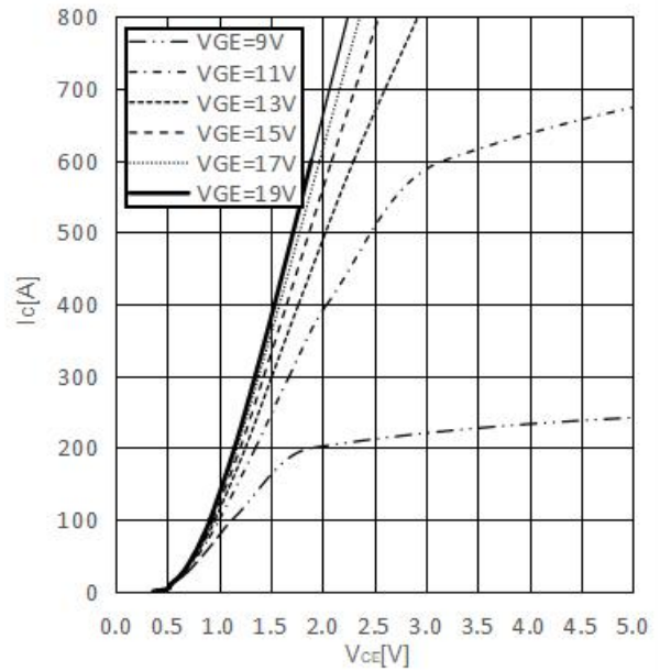
Output characteristic IGBT, Inverter (typical), Inclusive R_{CC+EE} IGBT 输出特性, 逆变 (典型值), 包含 R_{CC+EE} I_c = f(V_{CE}), T_{vj} = 150^\circ C
